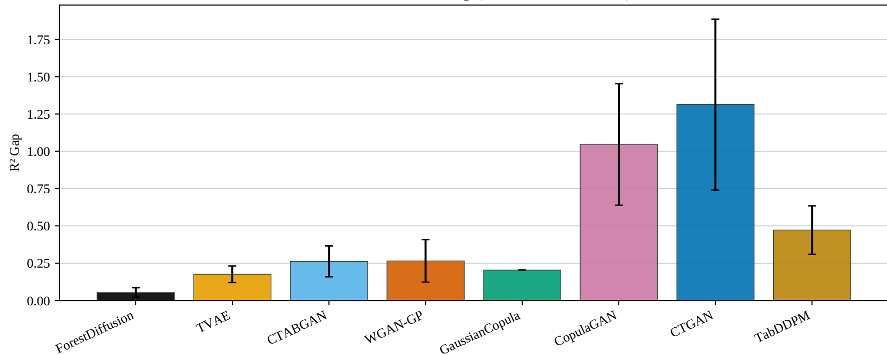
Real Estate — R^2 Gap (mean \pm SD, 10 seeds)
